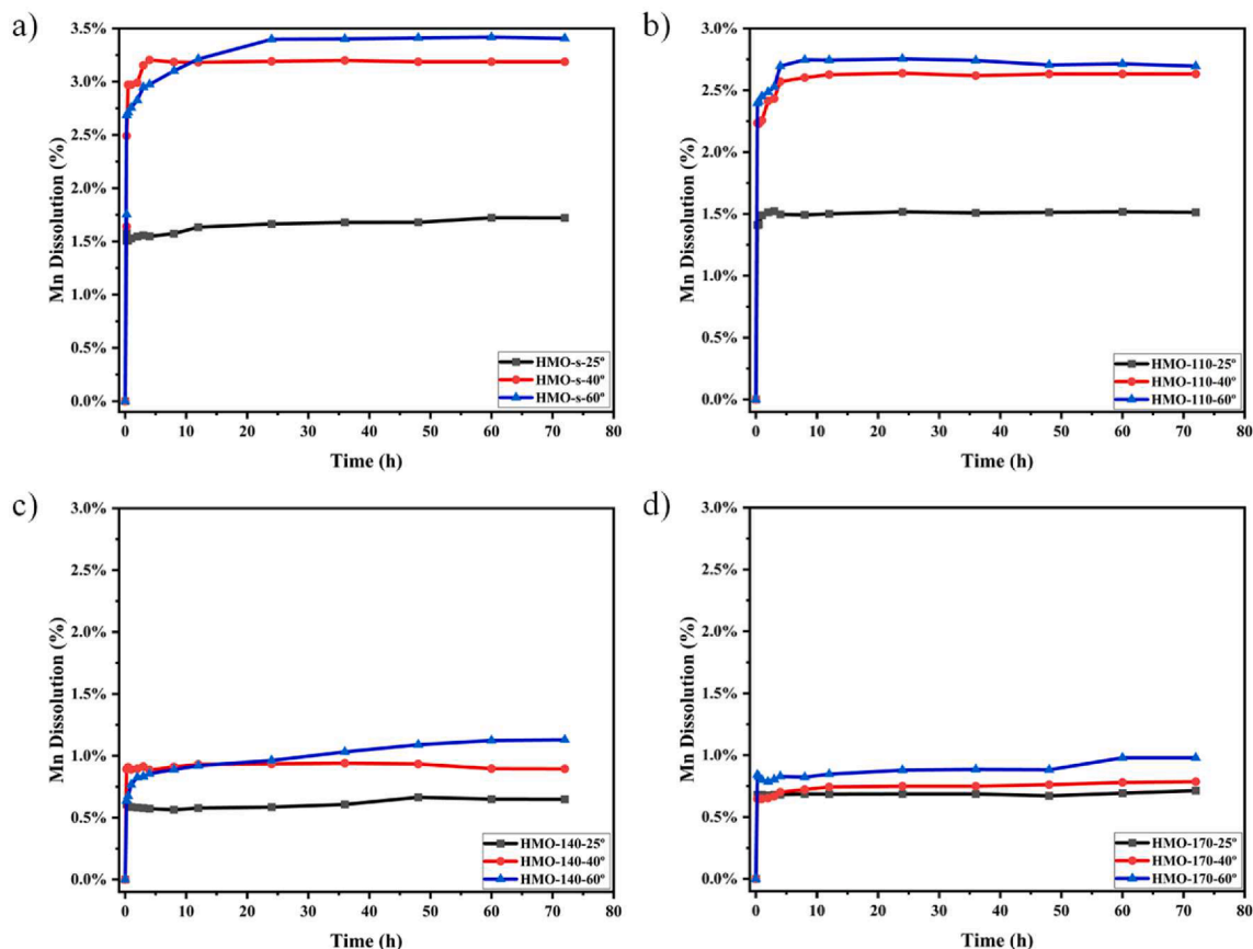
Fig. 9. Percentage of manganese dissolution at different temperatures. LMO-s (a), LMO-110 (b), LMO-140 (c) and LMO-170 (d).
